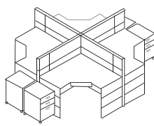
S-Type Workstation for Four Person Size 2850x1210x1140 mm(h)
