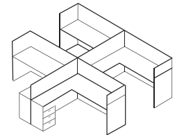
R-Type Workstation for Four Person Size 2410x1600x1220 mm (h)
