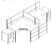
S-Type Workstation for Two Person Size 1425x1210x1140 mm(h)
