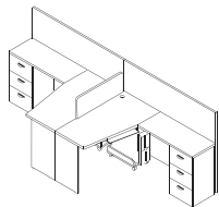
X-Type Workstation for Two Person Size 1205x3200x1220mm (h)
