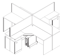
U-Type Workstation for Four Person Size 4000x3200x1200 mm (h)
