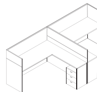
R-Type Workstation for Two Person Size 1205x1600x1220mm (h)
